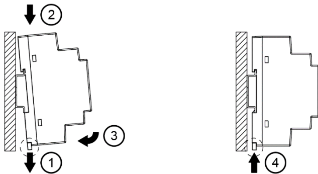
Fig. 2.1 Mounting
